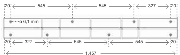
Hole pattern: Ground rail B
