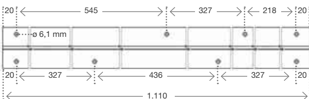
Hole pattern: Ground rail A
