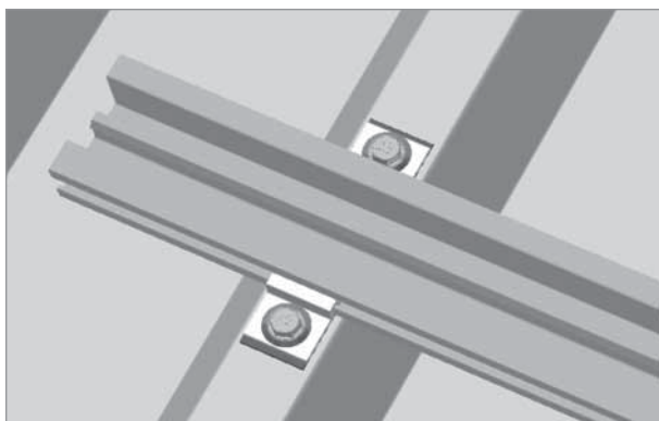
Mounted top trapezoidal fixation
