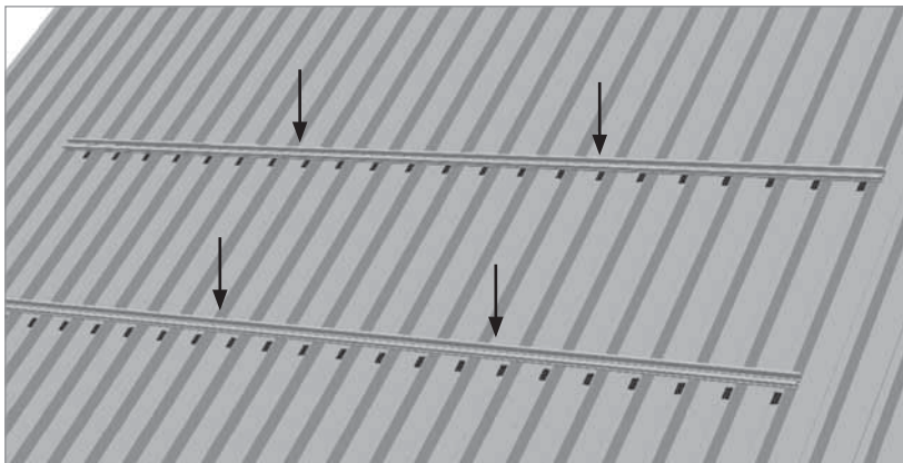
Aligning and placing the profiled rails
