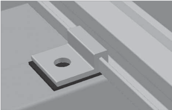
Correct fit of the trapezoidal top fixation
