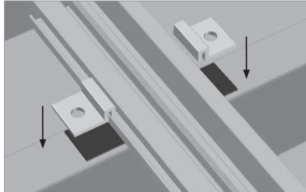
Positioning of the trapezoidal top fixations for bead heights < 20 mm
