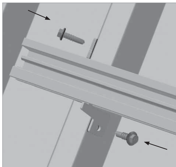
Positioning of the 6x25 mm drilling screw with a gasket
