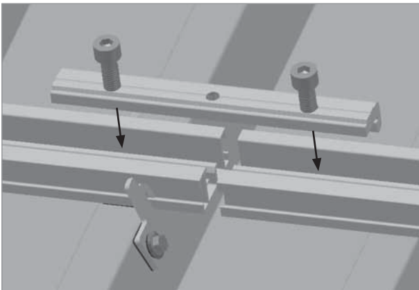
Profiled rail connection with Splice for framed PV modules
