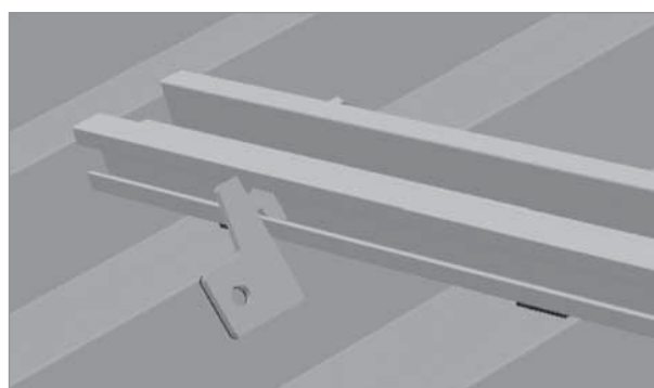
Positioning of the trapezoidal side fixation for bead heights \geq 20 mm
